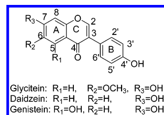
Figure 1. Soy isoflavone structures, substitution patterns, and numbering system.
